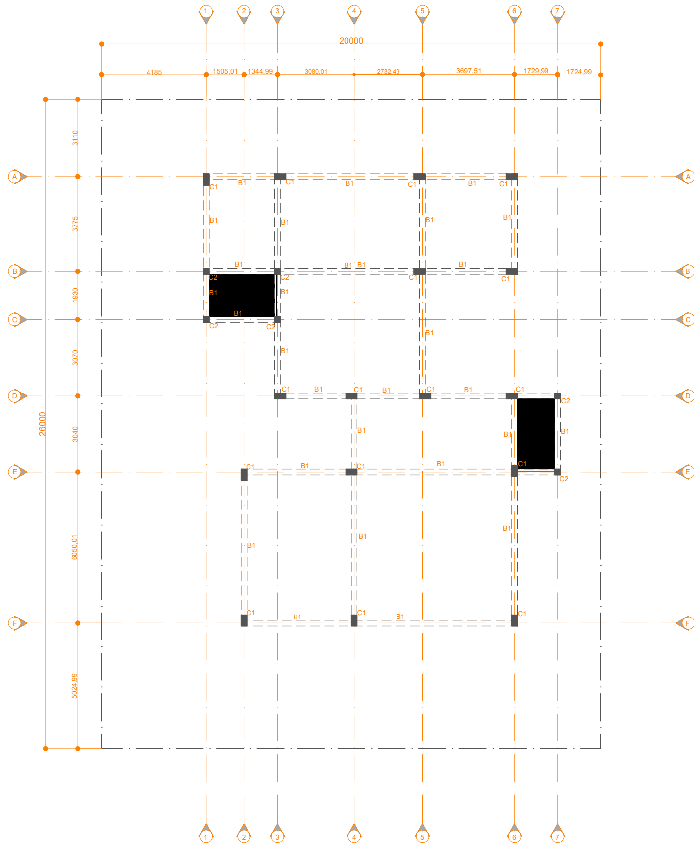
PLINTH BEAM PLAN
